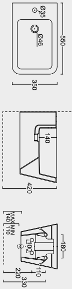
Cod. 31220101 Bidet sospeso Hide Square Hide Square wall hung bidet
